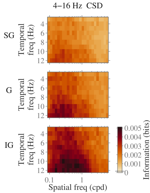
FIGURE 4.7. Information contained in the 4 Hz to 16 Hz CSD phase about different spatiotemporal components. The luminance of the movie was filtered in the spatial domain with using band-pass filters each with width one octave, and in the temporal domain with bandpass filters each with width 6 Hz. Datapoints are shown against the middle of the band on both x and y axes. Each row of panels corresponds to a different cortical depth, averaging over SG, G and IG compartments, respectively. Throughout all panels, the mean over 6 sessions is indicated. Statistical significance thresholds were computed for each datapoint individually, and a typical significance threshold is shown by the black line across the colour bar.
