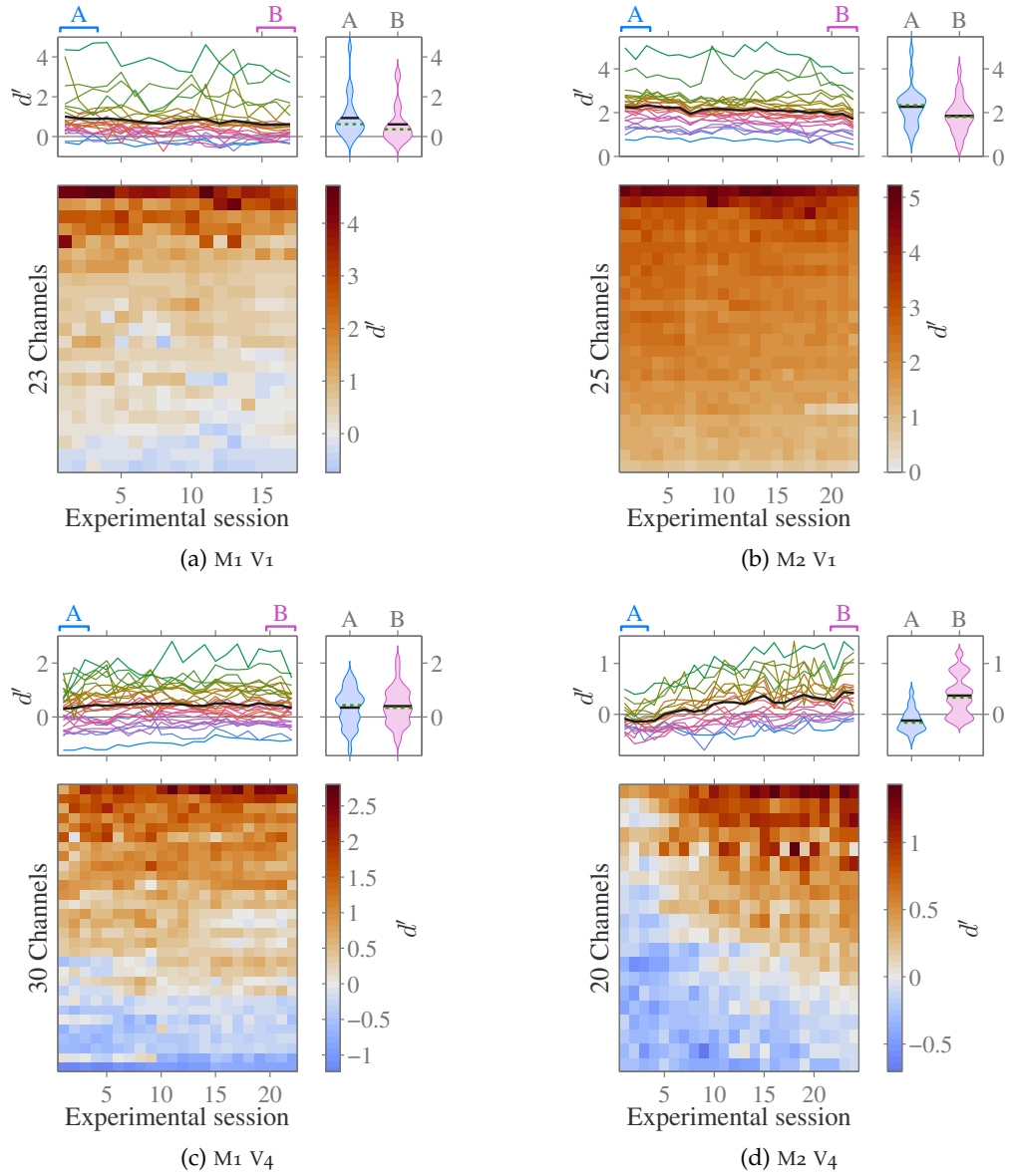
FIGURE 2.7. Change in sensitivity index, d' , over training sessions. (a): d' for M1 V1, shown for each recording channel, with channels ordered according to average d' over all sessions. Above, traces of d' for each channel (colours), and average over channels (black). Below, heatmap showing d' for each channel. Right top, violin plots showing distribution over channels of the average d' in the first (A) and last (B) three sessions, with mean (solid black line) and median (dashed green line) over channels indicated. The violin plot shows a Gaussian kernel density using a bandwidth determined automatically as described in Section 2.6.1. (b): Same as (a), but for M2. (c) and (d): Same as (a) and (b), but for V4.
