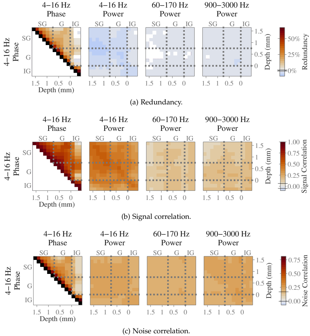
FIGURE 4.5. Redundancy of 4 Hz to 16 Hz CSD phase with 4 Hz to 16 Hz power, 60 Hz to 170 Hz power and MUA (900 Hz to 3000 Hz power). (a): Redundancy (as defined in Equation 3.3) between phase and power. Non-significant datapoints are shown in white, with median significance threshold (positive and negative) indicated by the black lines across the colour bar. (b): Signal correlation, reported as circular-circular correlation coefficient between phases and the circular-linear correlation coefficient between phase and power (see Section 4.1.3). Non-significant datapoints are shown in white, with minimum and maximum significance thresholds indicated by the black lines across the colour bar. (c): Same as (b), but for noise correlation instead of signal correlation.
