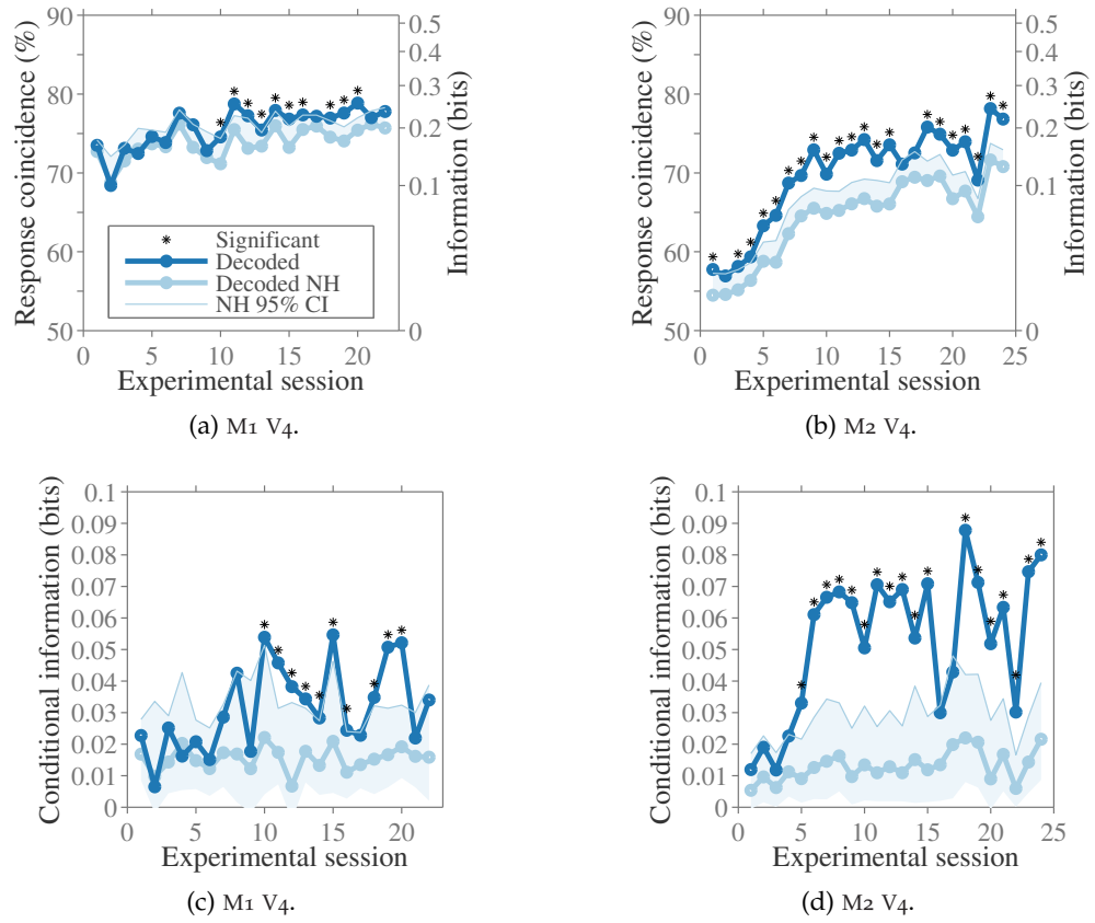
FIGURE 2.40. Response coincidence rate for V_4 . Same as Figure 2.39, but for V_4 .
