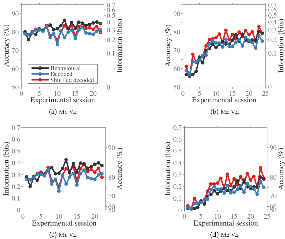
FIGURE 2.37. Classifying the stimulus group from V_4 population activity. We report the accuracy of the linear decoder classifying the group of each stimulus (greater or less than 30 % contrast) after training on the population activity (blue; (a) M_1 , 25 channels; (b) M_2 , 18 channels). For details, see caption of Figure 2.36.
