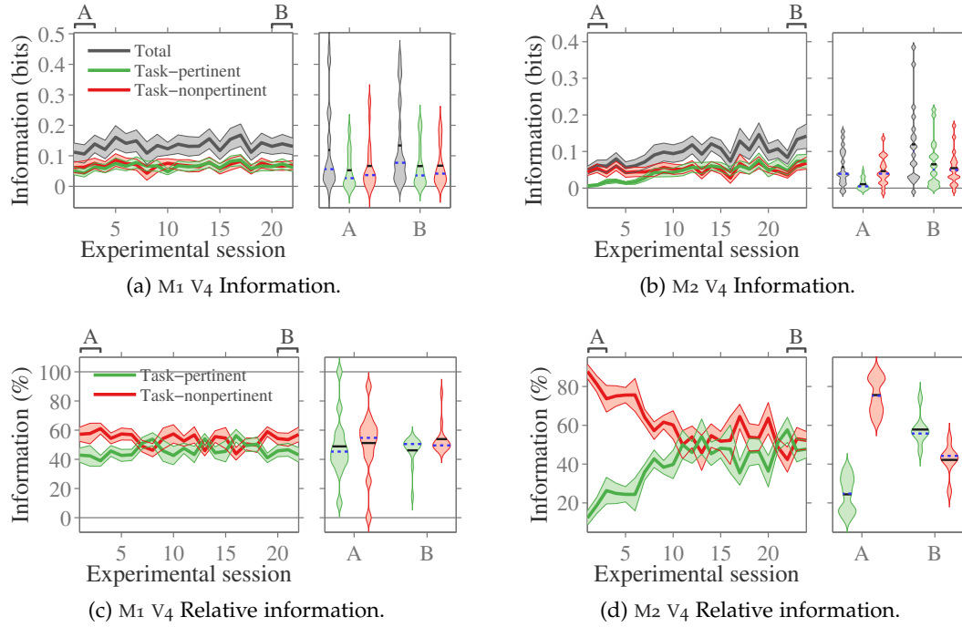
FIGURE 2.22. Breakdown of task-pertinent and nonpertinent information contained in V_4 recording channels. In (a) and (b), the total information about the stimulus (grey), task-pertinent information (green), and task-nonpertinent (red) contained in each of 25 and 18 channels respectively. In (c) and (d), the relative information about the stimulus which is task-pertinent (green) and task-nonpertinent (red) contained in channels with a significant amount of total information (13 and 7 respectively). Main panels: across training sessions, the average information over channels, with standard error across channels indicated by the shaded region. Right hand panels: distribution over channels of the information (or relative information) in the first three sessions (A) versus last three sessions (B), with mean (solid black line) and median (dashed blue line) over channels indicated. The violin plot shows a Gaussian kernel density, using a bandwidth determined as described in Section 2.8.1. The PT bias correction method was used, with the residual bias further reduced using bootstrapping (see Section 2.8.5.2). The stimulus class imbalance was corrected using subsampling, as described in Section 2.8.4.
