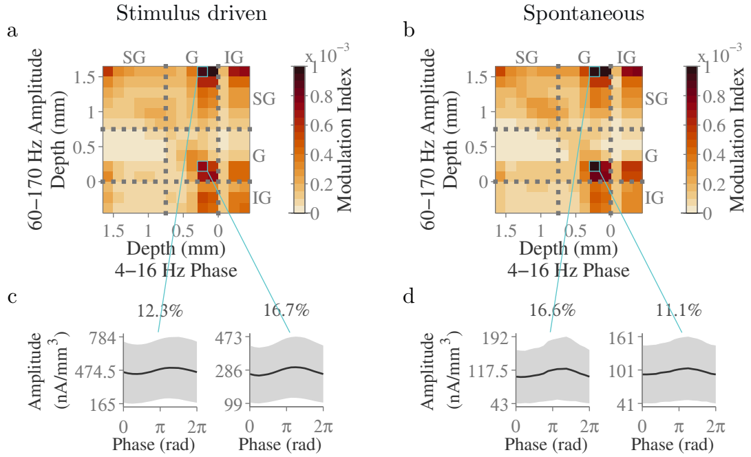
FIGURE 4.10. Cross-frequency phase–amplitude coupling . Phase–amplitude modulation index between low frequency (4 Hz to 16 Hz) phase and high frequency (60 Hz to 170 Hz) amplitude ((a): movie driven activity; (b): spontaneous activity). Mean of 5 sessions. (c) and (d): Amplitude as a function of binned phase for a typical example session (F10nm1), for IG→IG coupling (left) and IG→SG coupling (right).
